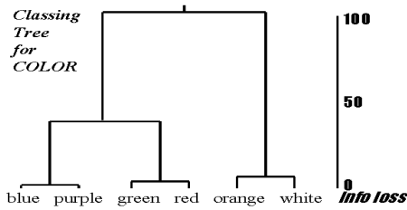
Figure 8: Classing Tree with Information Loss Measure
