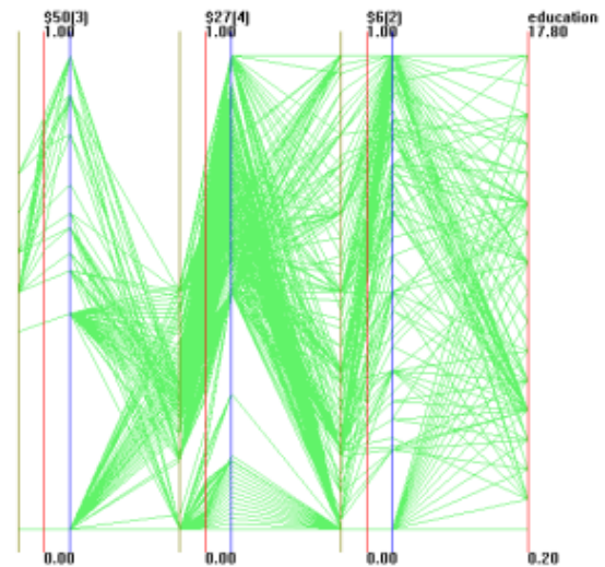
Figure 7: LDOD display using the Three-Axes Method. The green axis represents the minimum within the dimension cluster and the blue axis corresponds to the maximum.
