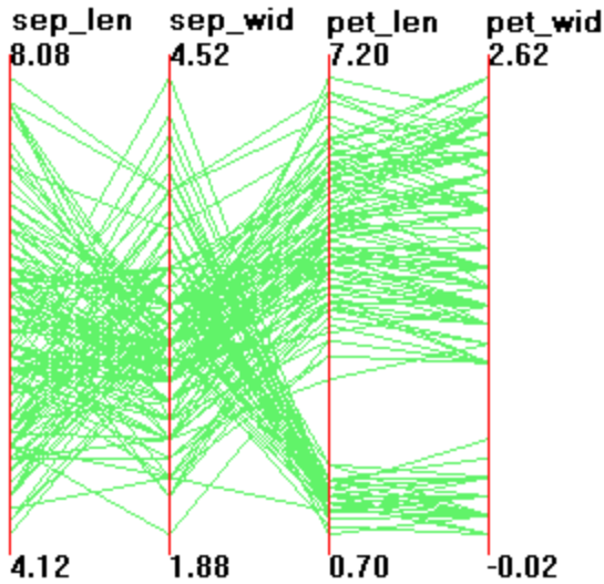
Figure 1: Iris data set (4 dimensions, 150 data items) in Parallel Coordinates. Individual data items can be seen clearly.
