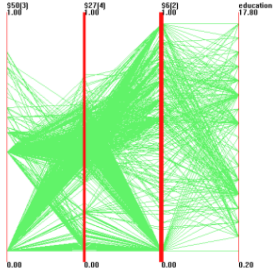
Figure 6: An LD space of the Census Dataset constructed of 4 dimension clusters. These clusters are composed of 3, 4, 2, and 1 original dimensions respectively from left to right of the displays. The GDODs are shown using the Axis Width Method.
