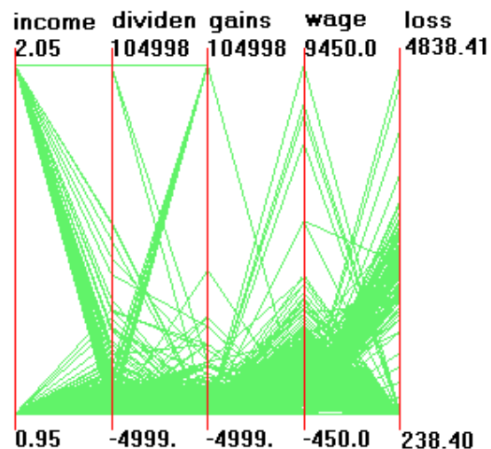
Figure 10: The lower dimensional subspaces generated by VHDR.
