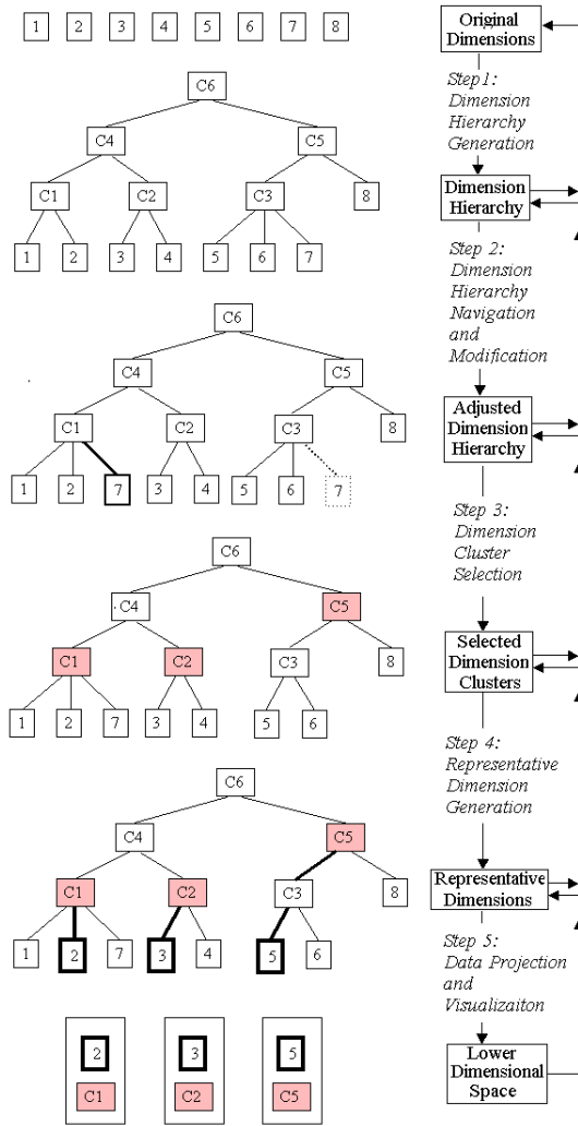
Figure 3: System structure of VHDR.
